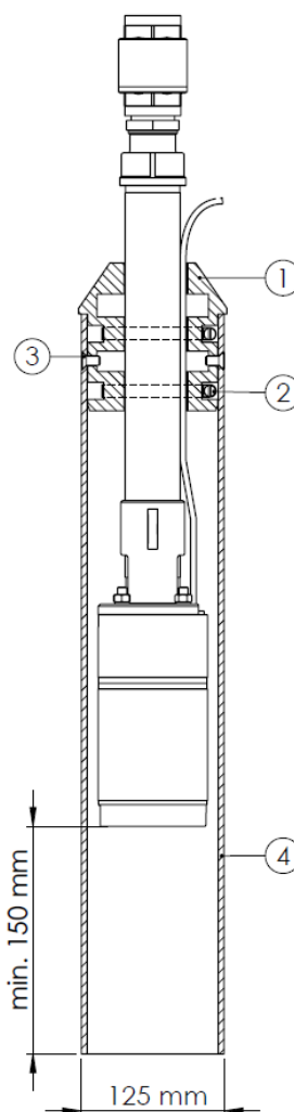
sample flow sleeve
